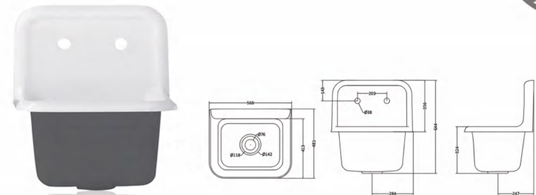
NH-RT001 22" L 560 x W 460 x H 660/320MM
