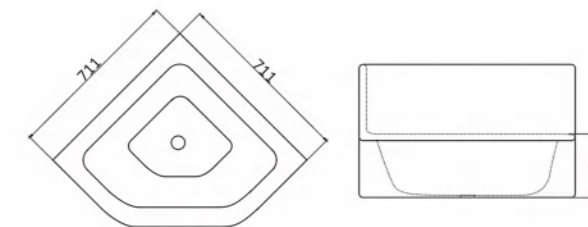
NH-8003 L 711 x W 711 x H 190MM Floor-mounted corner sink Optional coated wire rim guard
