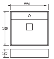
PB2029 尺寸：550x500x120mm
