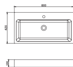
PB2143 尺寸：800x420x100mm
