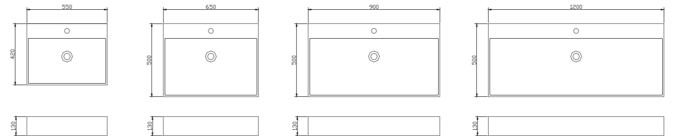
PB2212 550x420x130mm PB2213 650x500x130mm PB2214 900x500x130mm PB2215 1200x500x130mm
