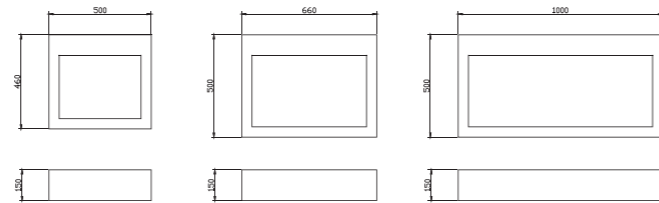
PB2209 500x460x150mm PB2210 660x500x150mm PB2211 1000x500x150mm
