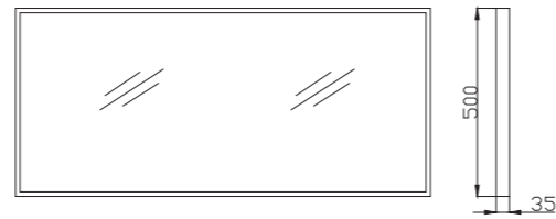
PB4311 尺寸: (from 800 to 1800)X500X35mm
