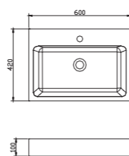
PB2142 尺寸：600x420x100mm
