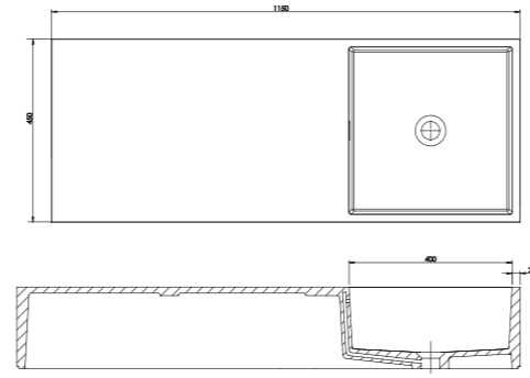
PB2227 550x450x200 mm PB2228 850x450x200 mm PB2229 1150x450x200 mm
