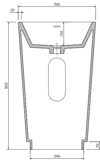
PB2195 尺寸: 500x450x820mm
