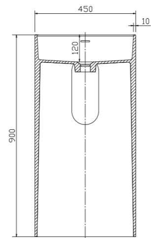
PB2208 尺寸: \varnothing 450 \times (820 \sim 900) mm
