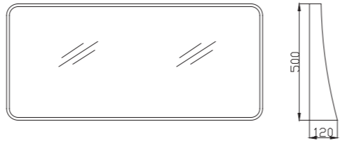
PB4310 尺寸: (from 800 to 1800)X500X120mm
