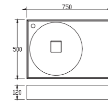
PB2027 尺寸：750x500x120mm
